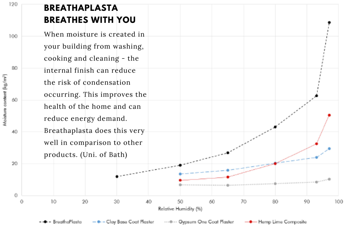
Figure 4 Isotherm comparison (moisture mass per unit volume)
